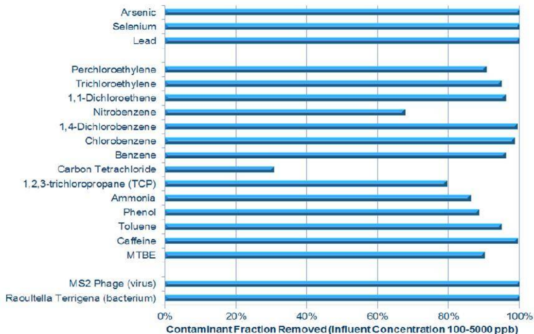
Shield 500 Performance @ 500 gal/day
